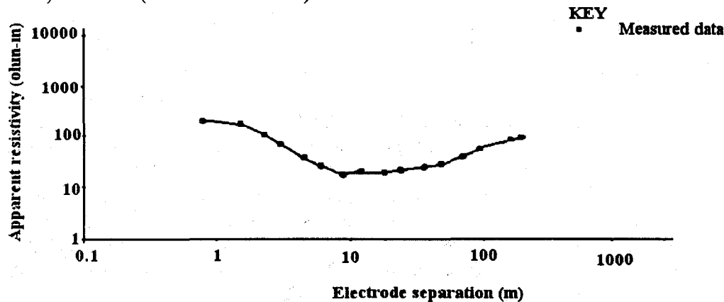
Fig. 4. Vertical Electrical Sounding (VES) curve from Oforikrom near Techiman
